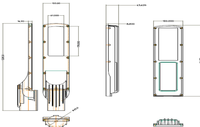
NOMINAL DIMENSIONS IN mm Tolerance +/-5
